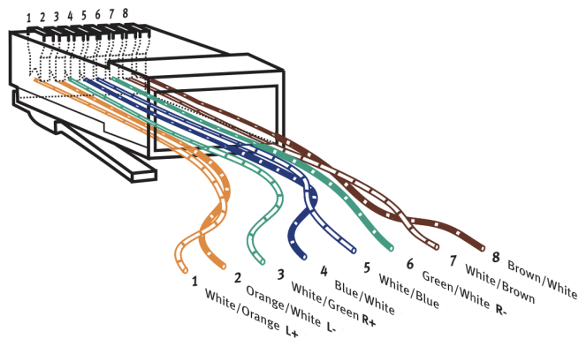
StudioHub+ pinout.
