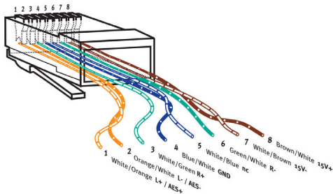
StudioHub+ Universal Pinout Reference
